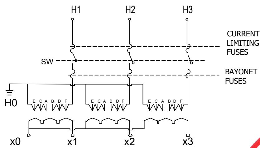
WIRING DIAGRAM
